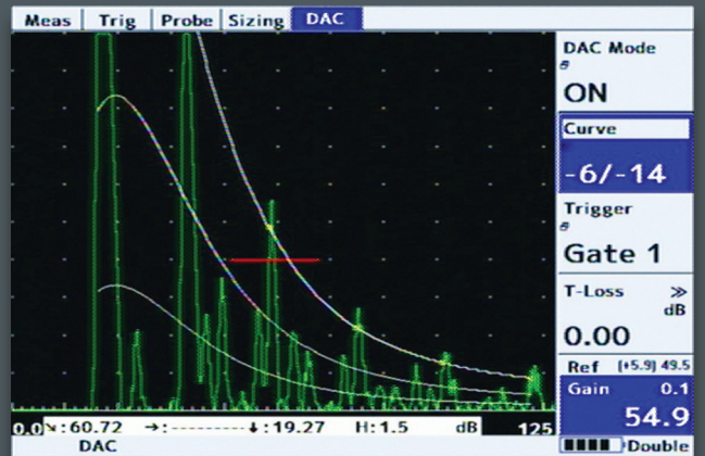
Dynamic DAC
