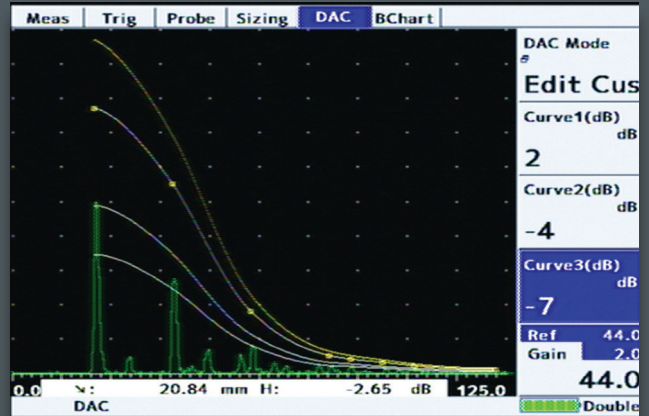
Customisable DAC
